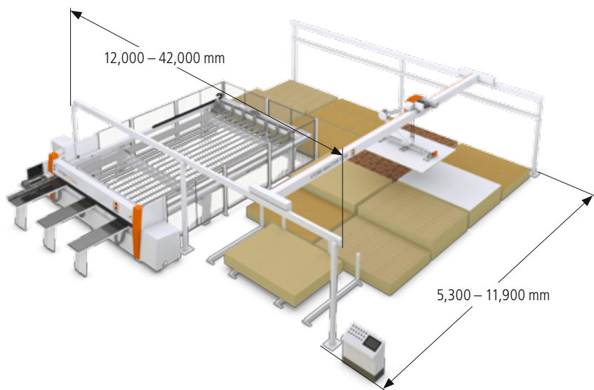
STORE-MASTER 5110 Panel Storage System with TECTRA 6120 dynamic and control terminal at emplacement spot.
